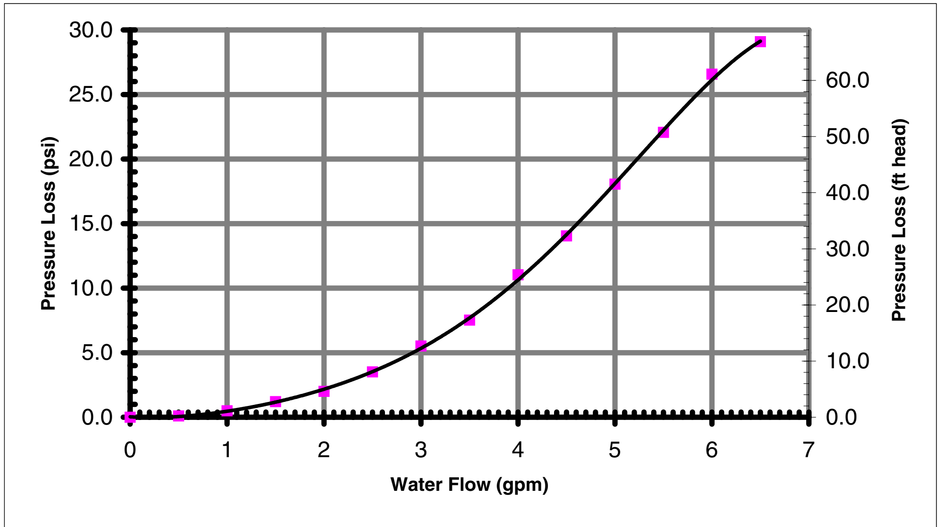
Continuum 2424 and Continuum 2402 Pressure Drop Curves Pressure Loss vs. Water Flow
