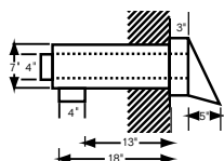
FT-4 Concentric Pipe-in-Pipe Termination
