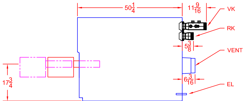
SIDE VIEW
