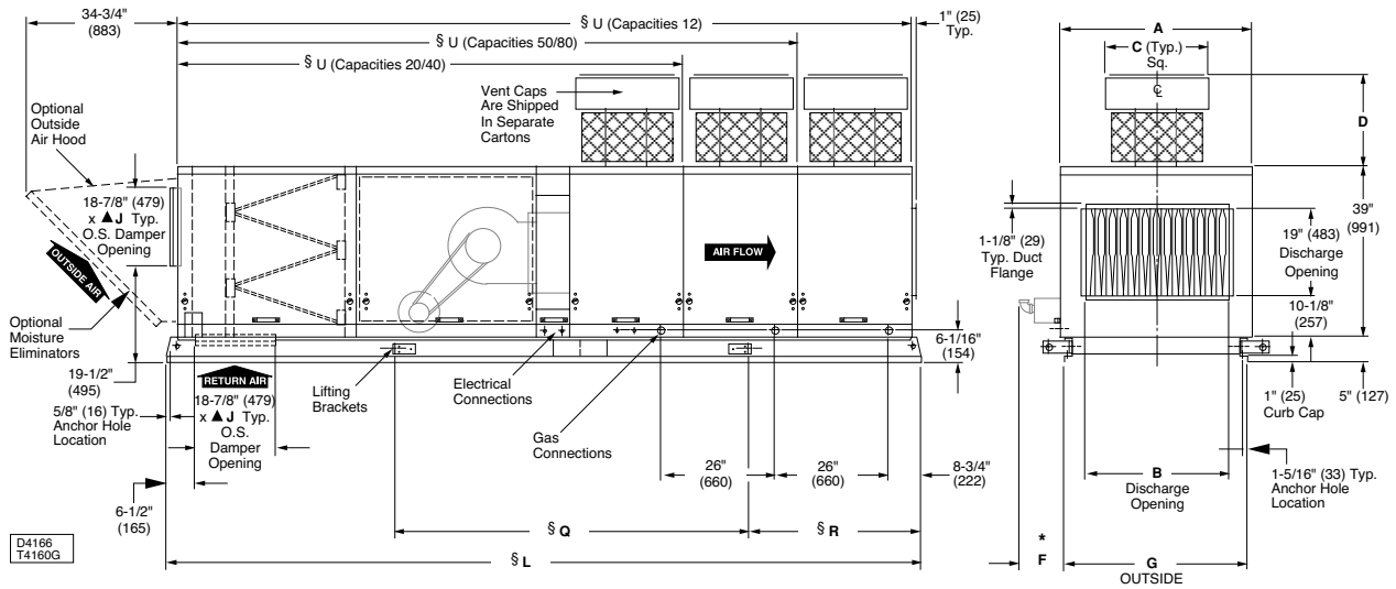
Rooftop Arrangement [RA] "G" Capacities [CA] 20 - 12 Unit Sizes Capacity 12 shown
