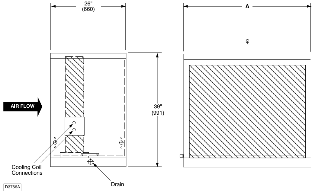
Coil Cabinet Module† Capacities [CA] 10 - 80 Unit Sizes (Right hand service access shown)
