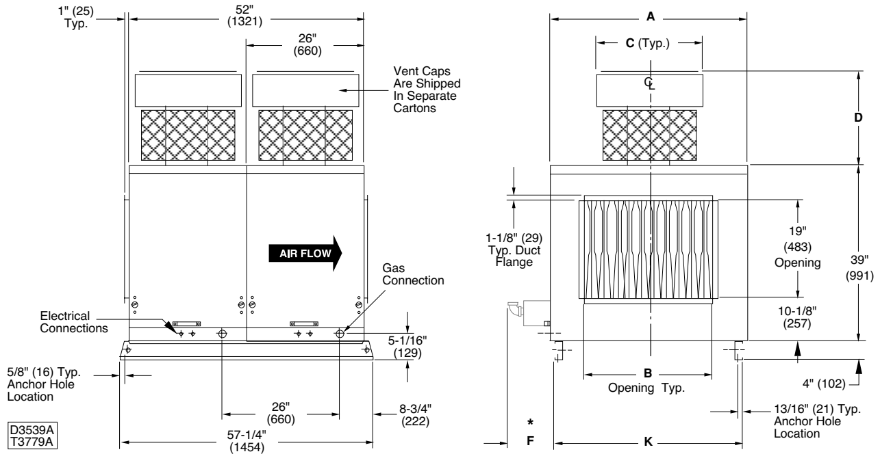
Rooftop Arrangement [RA] "A" Capacities [CA] 50 - 80 Unit Sizes
