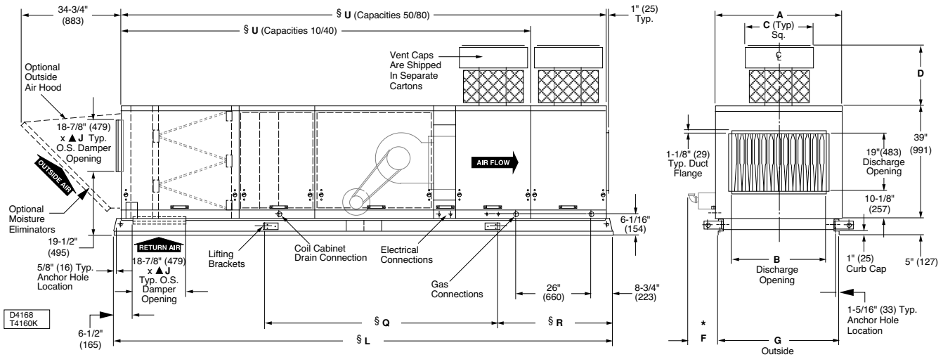
Rooftop Arrangement [RA] "K" Capacities [CA] 10 - 80 Unit Sizes Capacity 50 - 80 shown
