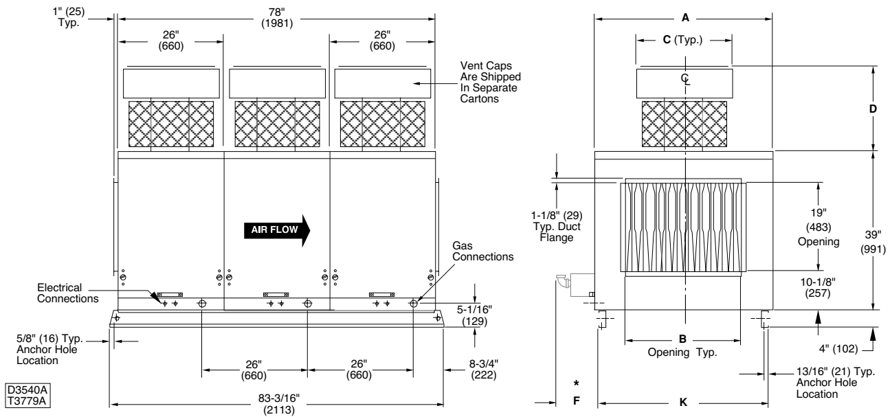
Rooftop Arrangement [RA] "A" Capacity [CA] 12 Unit Sizes
