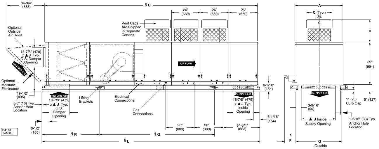
Rooftop Arrangement [RA] “J” Capacities [CA] 20 - 12 Unit Sizes Capacity 12 shown
