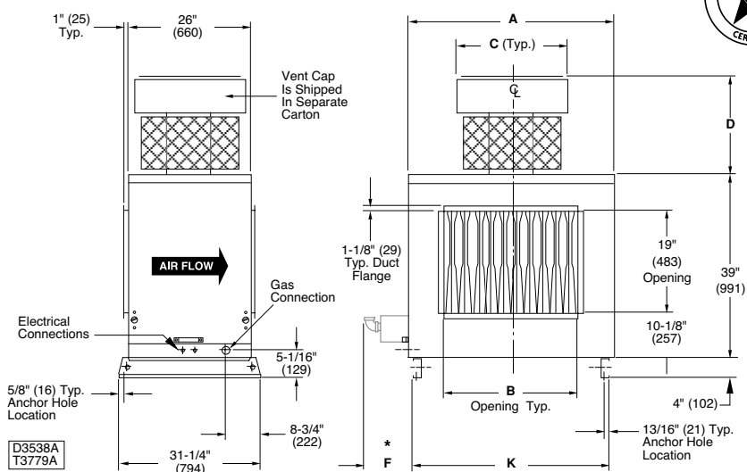
Rooftop Arrangement [RA] "A" - Capacities [CA] 10 - 40 QVRT - 100/400 MBH Unit Sizes
