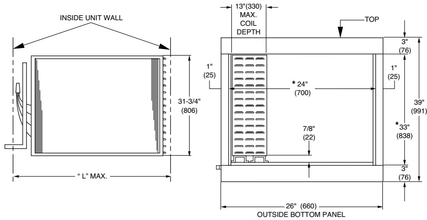
MAXIMUM COIL DIMENSIONS
