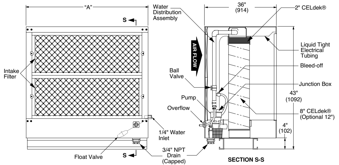
Evaporative Cooler Module Capacities [CA] 10 - 80 Unit Sizes
