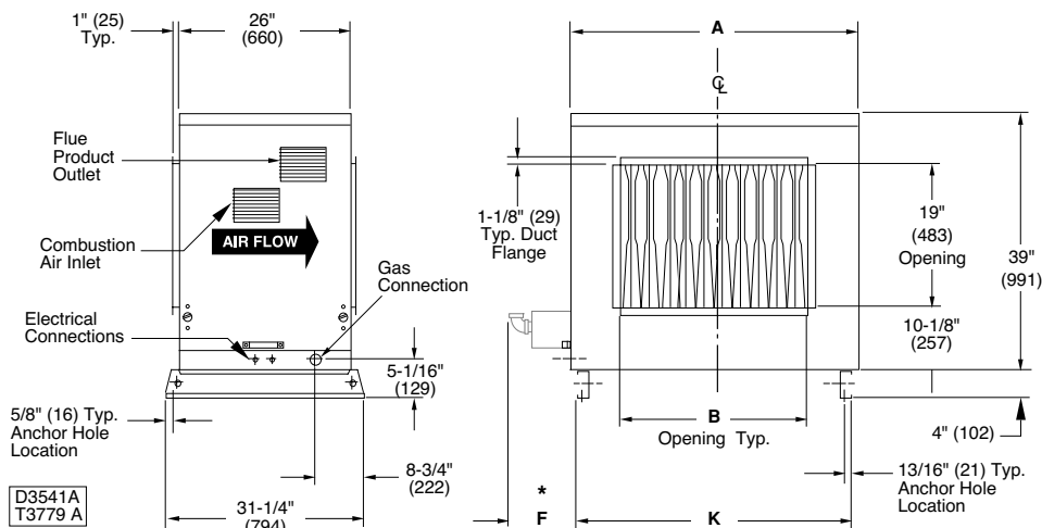
Rooftop Arrangement [RA] "A" - Capacities [CA] 10 - 40 QVPV - 100/400 MBH Unit Sizes
