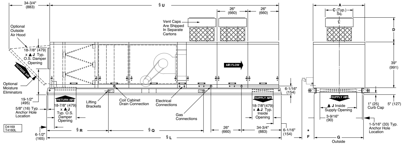
Rooftop Arrangement [RA] "L" Capacities [CA] 10 - 80 Unit Sizes Capacity 50 - 80 shown
