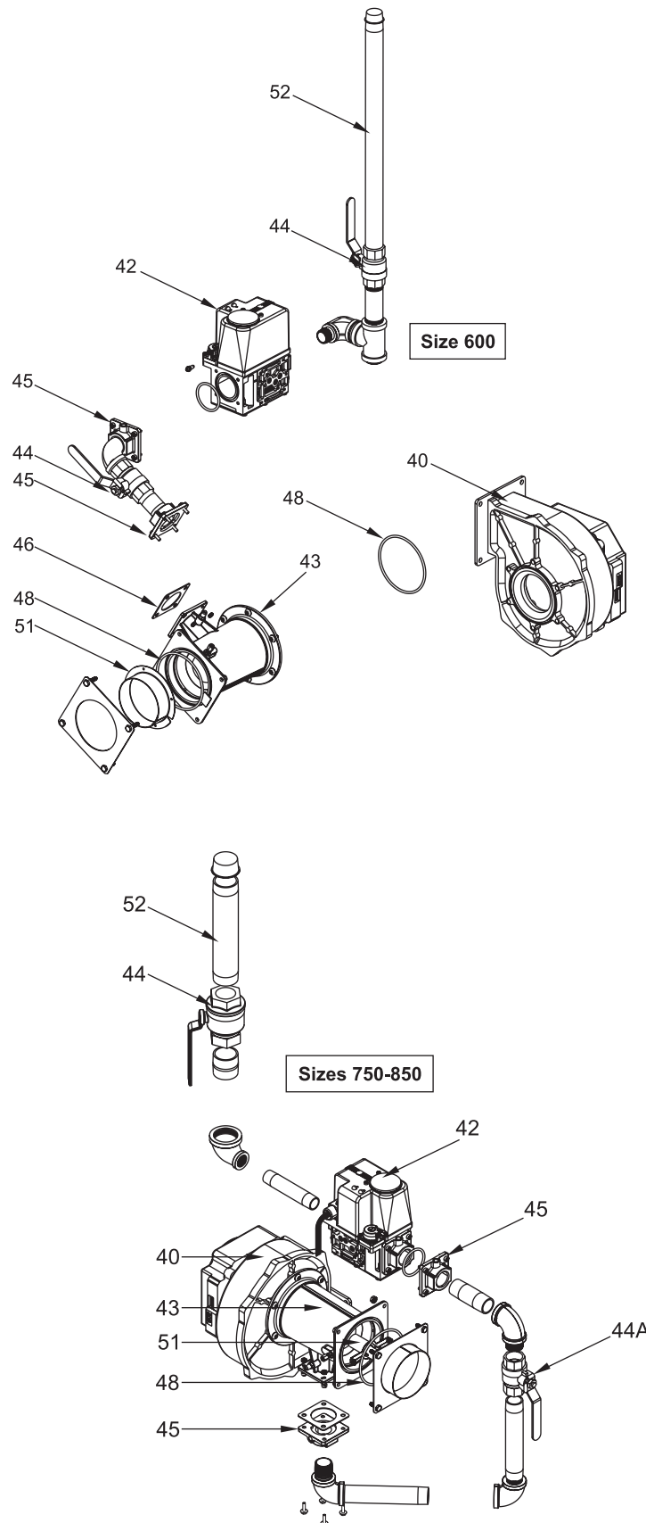
Figure 52b - Gas Train Components, Sizes 600-850
