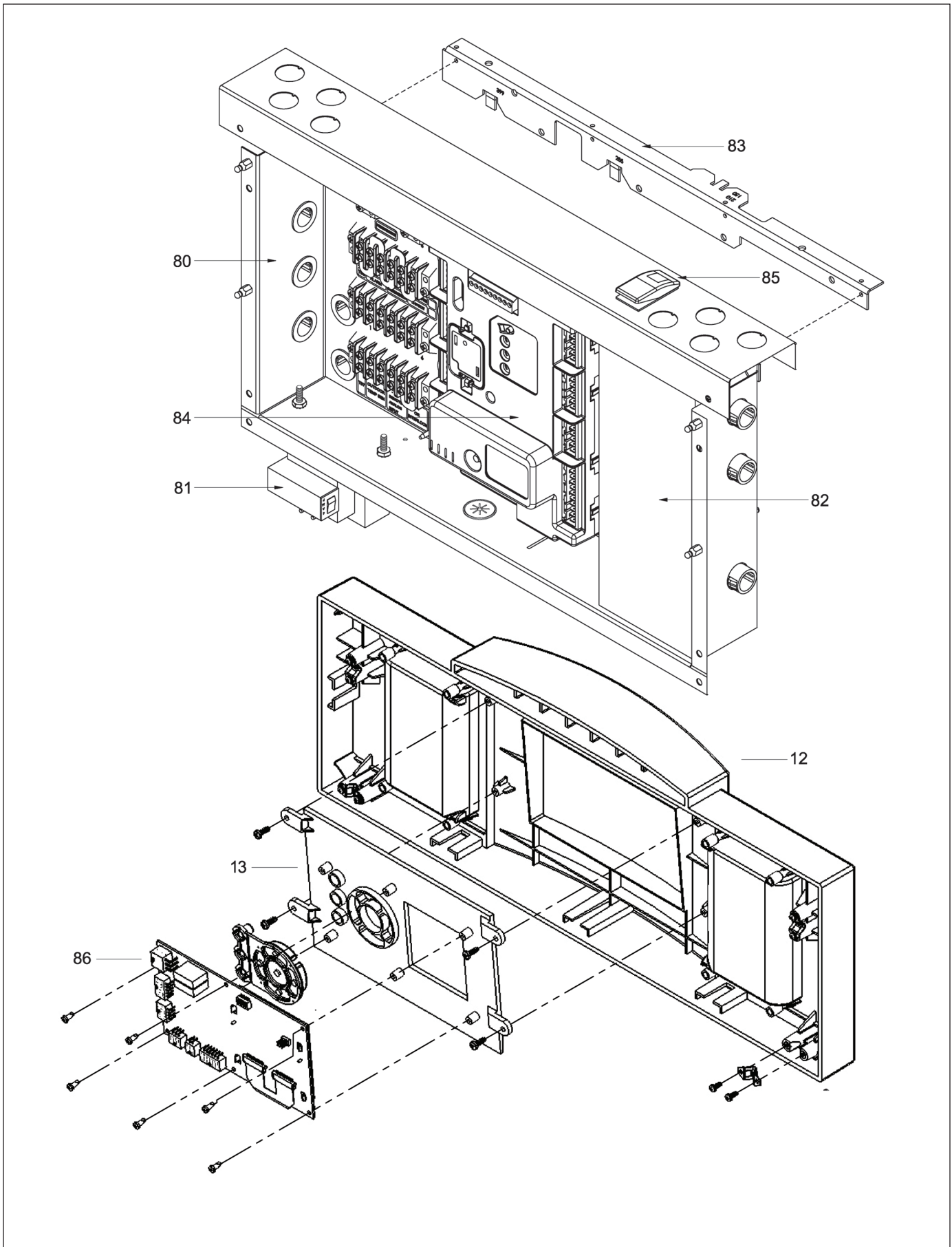
Figure 54 - Electrical Components
