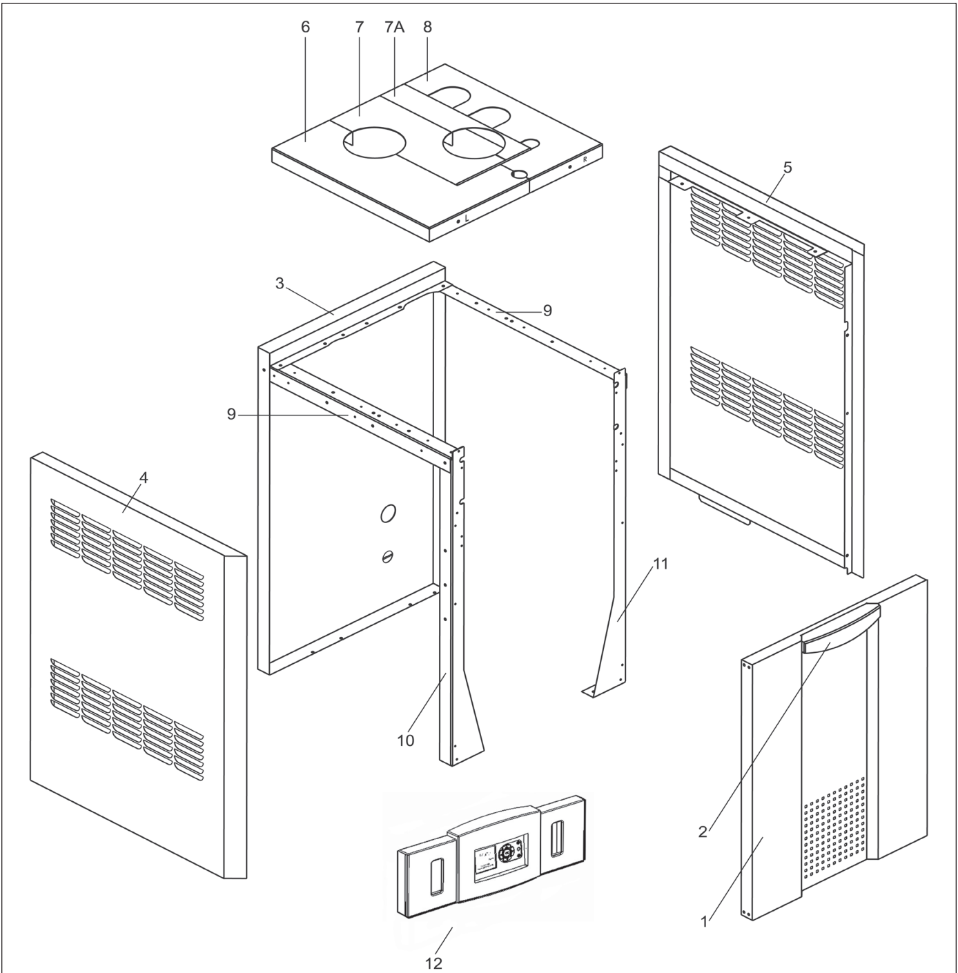
Figure 50 - Jacket Components
