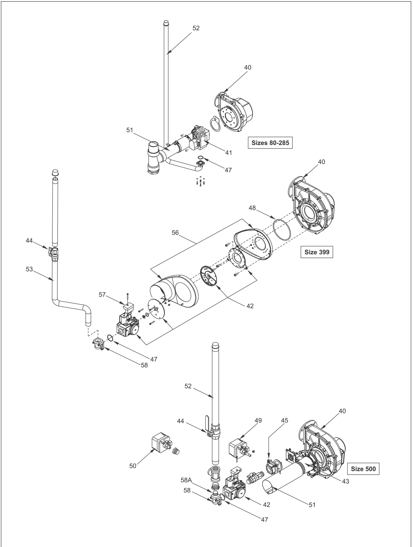
Figure 52a - Gas Train Components, Sizes 80-500
