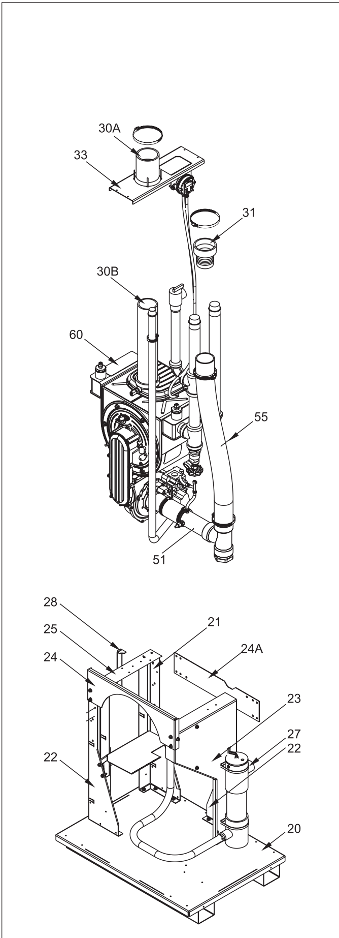
Figure 51a - Internal Components, Sizes 80-210
