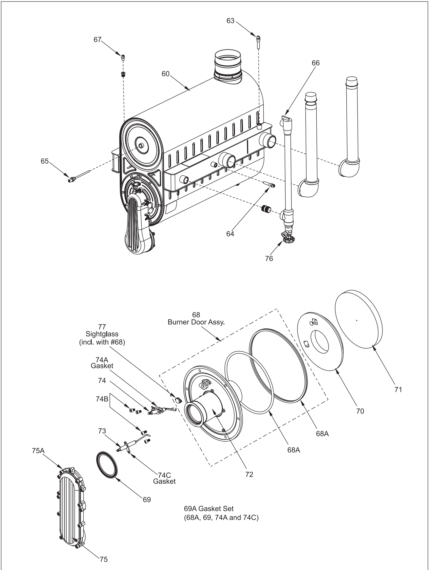
Figure 53 - Heat Exchanger Components
