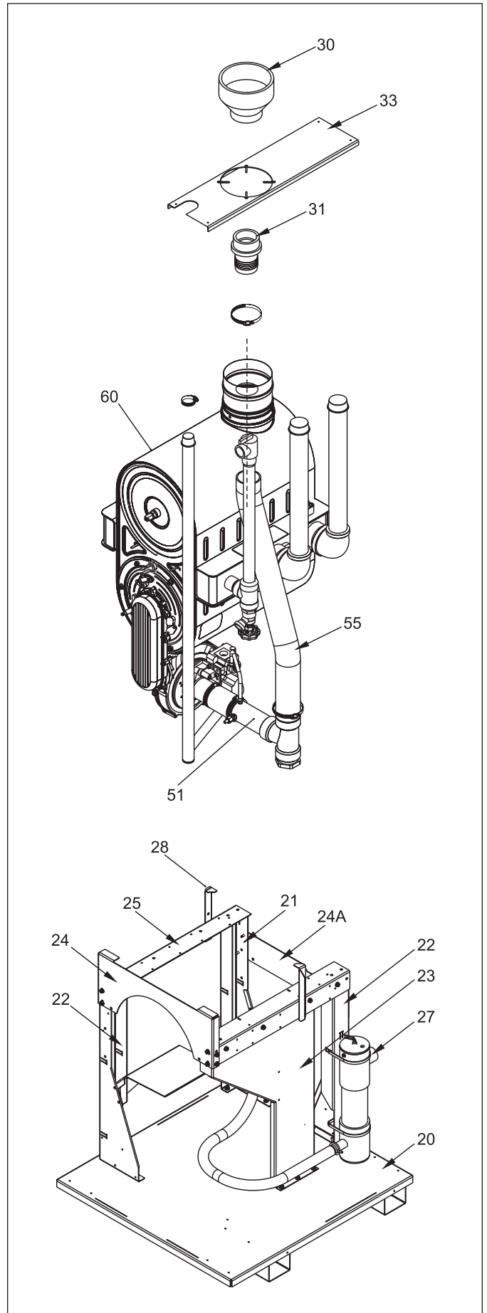
Figure 51b - Internal Components, Sizes 285-600
