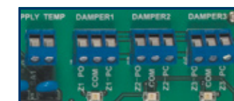
Easy to wire terminals and damper position LEDs for quick installation and check out
