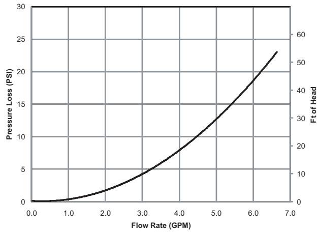
Pressure Loss
