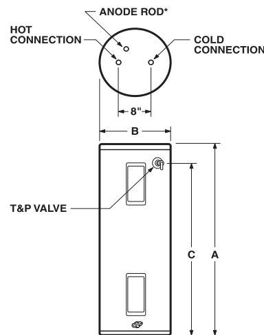
*Location for optional top-mounted T&P Valve, if available and ordered from factory.
