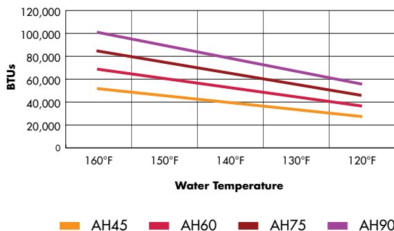
Heating Capacity Chart
