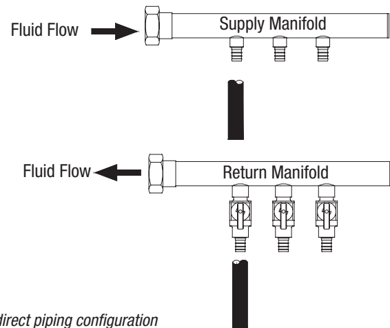
direct piping configuration
