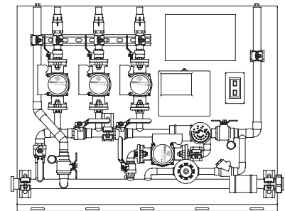
D-VIP Hybrid panel.
