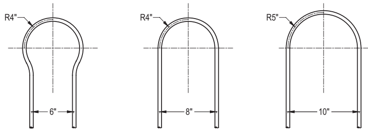
bend radius for RadiantPEX tubing
