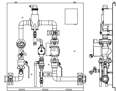
P-Series Primary Panel.
