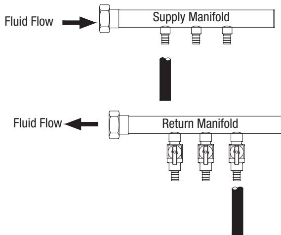
tubing reverse-return piping configuration
