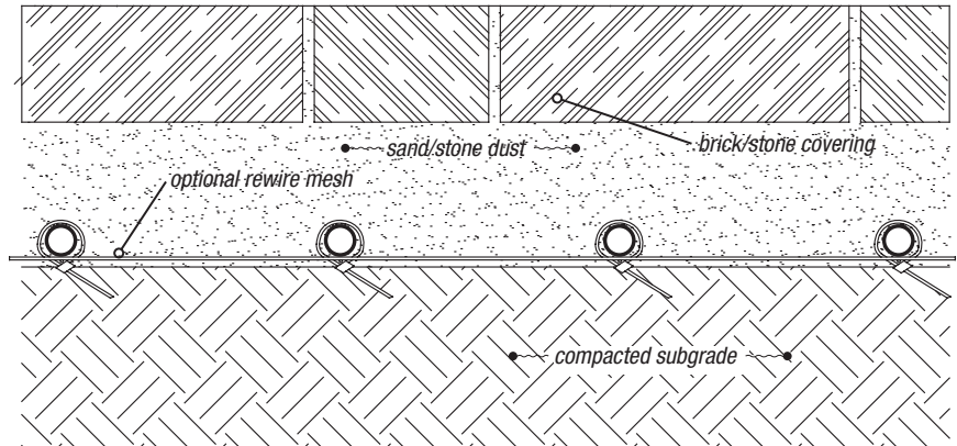
rewire may be used to help secure tubing before the sand/stone dust layer is added.
