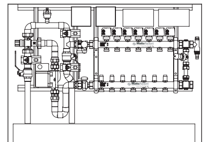
Z-Panel with circulator and mix valve.
