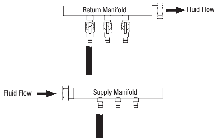
manifold reverse-return piping configuration
